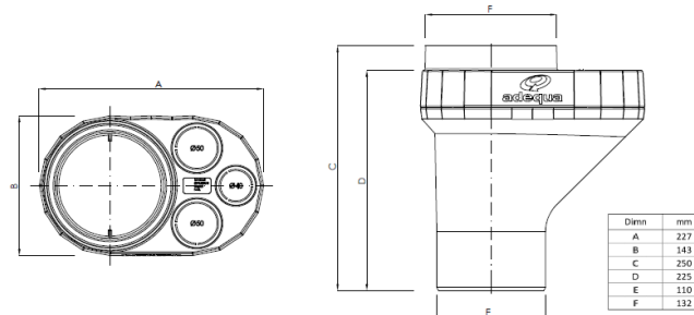
Figure 2 - DN 110
